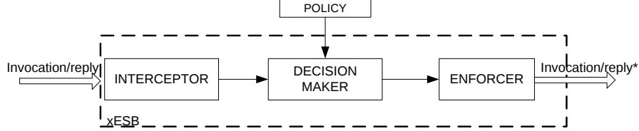
Fig. 2. The enforcement process behind xESB
