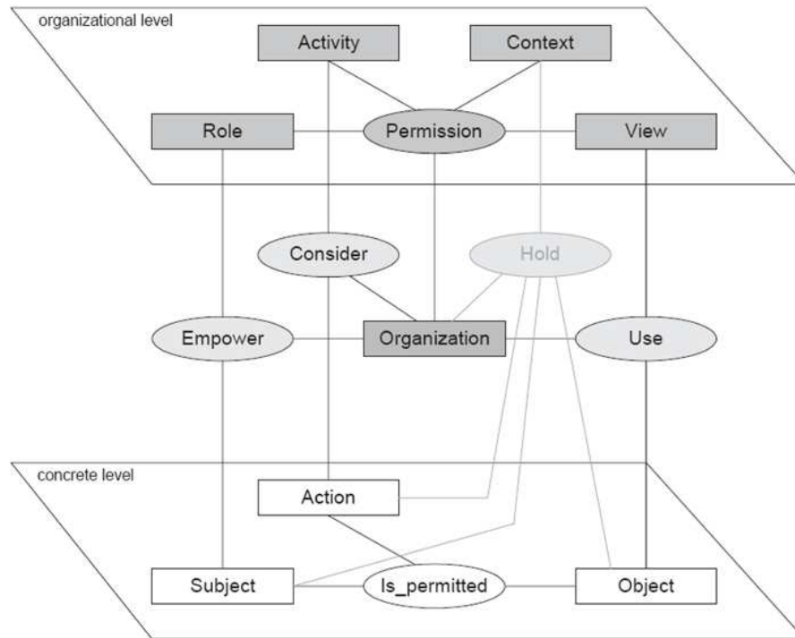
Fig. 3. The OrBAC Model (taken from [16])
