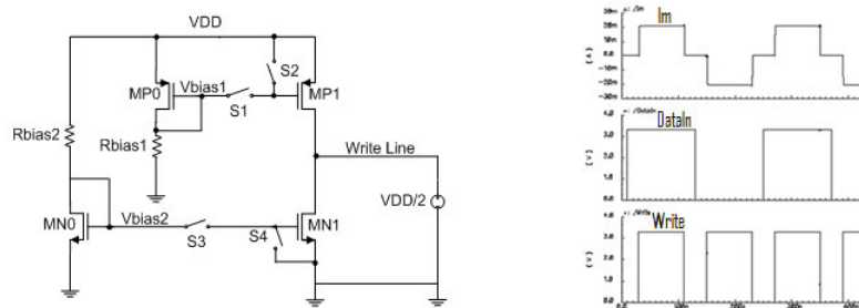
Fig. 6. Left: Bidirectional current generator. Right: Bidirectional current generator electrical behavior.
