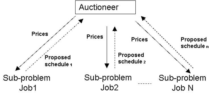
Fig. 3. Problem-solution schema
