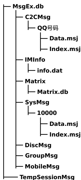
Figure 2. MsgEx.db data structure.
