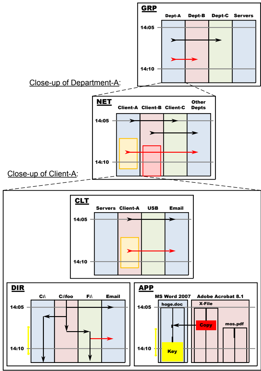
Figure 10. Analytic workflow.
