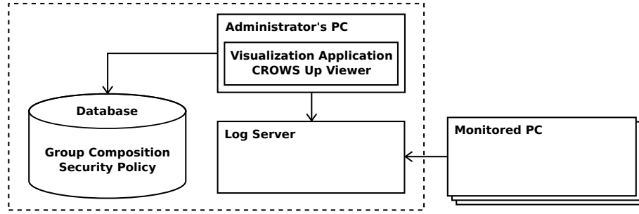
Figure 3. System architecture.
