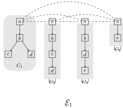
Fig. 1: A Labeled Event Structure and its maximal configurations.
