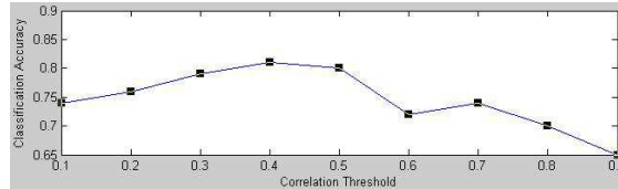
Fig.1. Recognition accuracy with different choices of correlation threshold.
