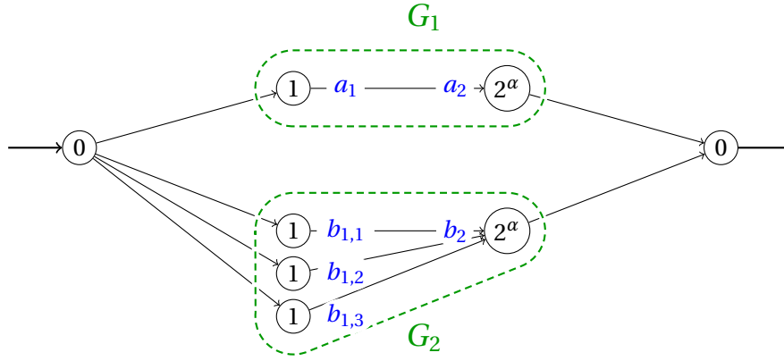
Figure 4: Series-parallel graph of the counter example.
