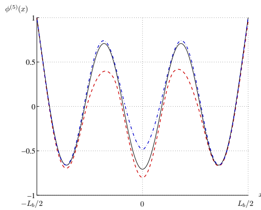
Fig. 3. Fifth mode shape for the structures (S1) (in dashed line), (S2) (in dash-dotted line) and the bare beam (solid line).
