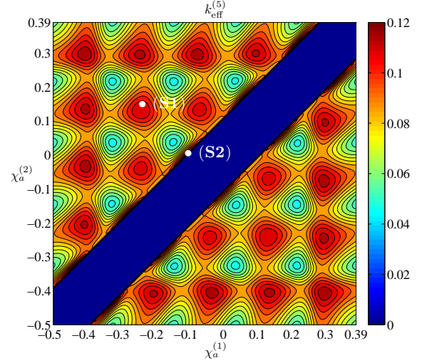
Fig. 2. EEMCC for the fifth flexural mode shape.
