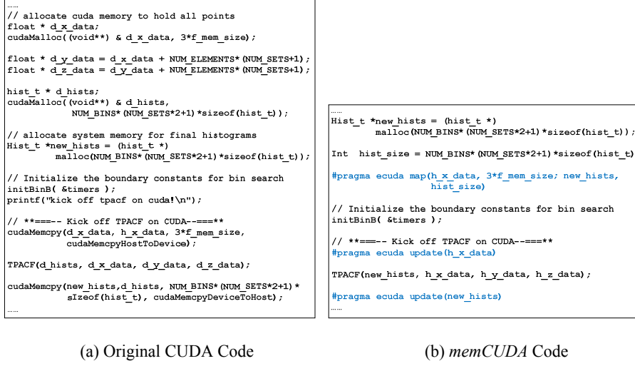
Fig. 4. Original CUDA code vs memCUDA TPACF code
