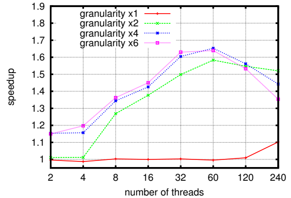
Fig. 12: Xeon Phi speedup with varying granularities
