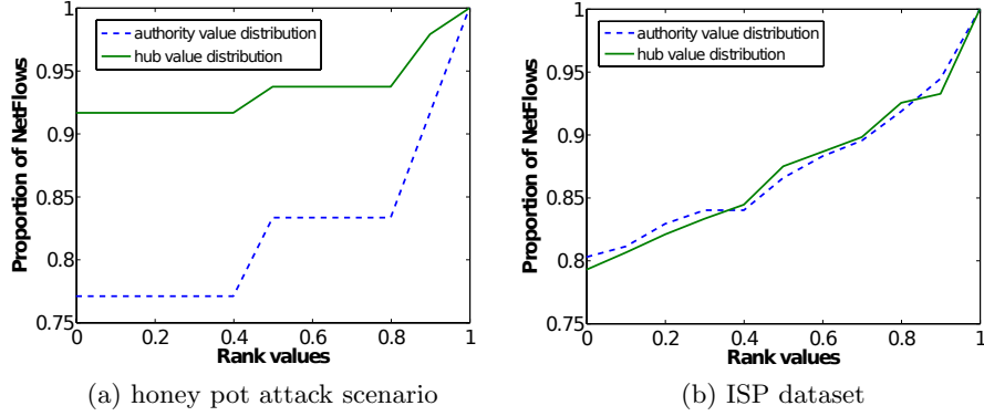
Fig. 5: NetFlow ranks cumulative histogram
