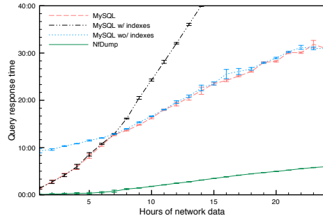
Fig. 1. Listing queries
