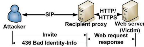
Fig. 2. The testbed for measuring resource consumption
