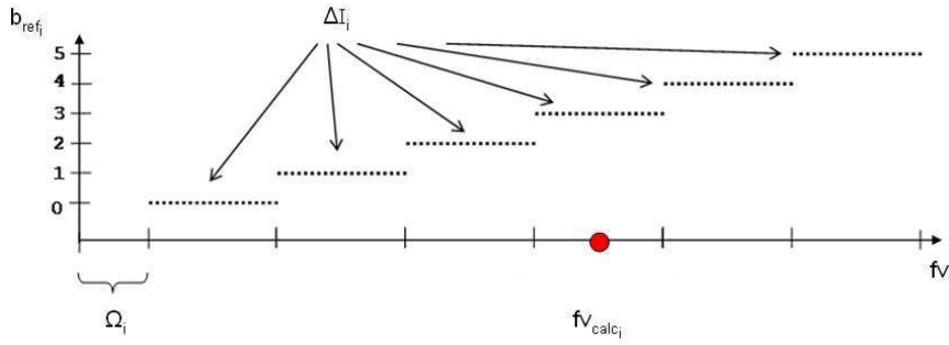
Fig. 2 Example of backward calculation (reverse mapping) of a feature vector element fv_{calc,i} based on the corresponding reference BioHash b_{ref,i} , Interval Length \Delta I_i and Interval Offset \Omega_i .
