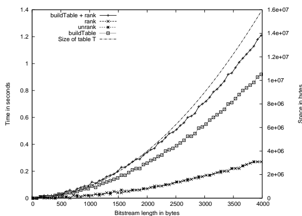
Fig. 4. Space and time of RtE
