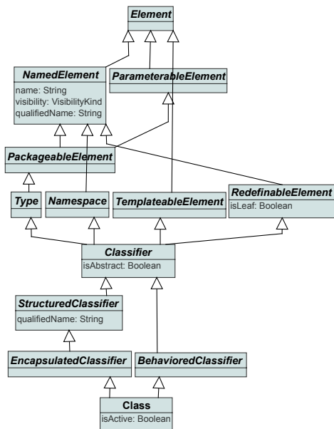
Fig. 3. The super inheritance tree of the UML class Class
