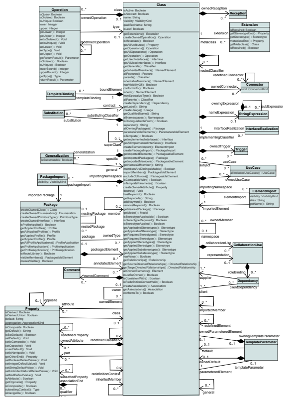
Fig. 6. Flattening of the UML class Class followed by a slicing parameterized with a radius of 1
