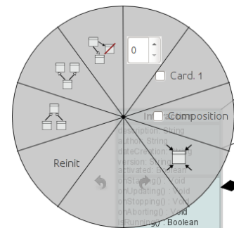
Fig. 5. The piemenu activated by clicking on a class to apply filters.
