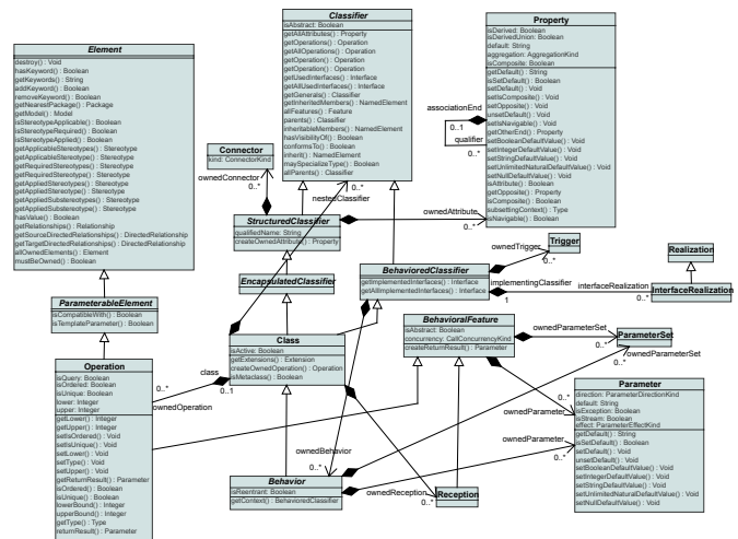
Fig. 4. Slicing the UML metamodel using the class Class as input and parameterized with a radius of 3 and by slicing composition references only
