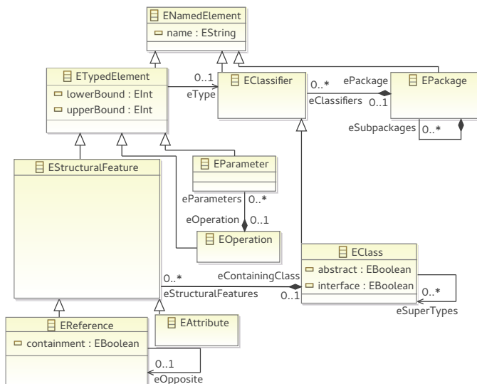
Fig. 2. An example of metamodel: an excerpt of the Ecore metamodel
