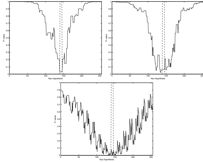
Fig. 3. Returned P-values plotted for all possible values for one byte for s = 3, 5, 15 (top left, top right and bottom middle respectively). The dashed lines represent the boundaries identified by the minimum and maximum observed fault.
