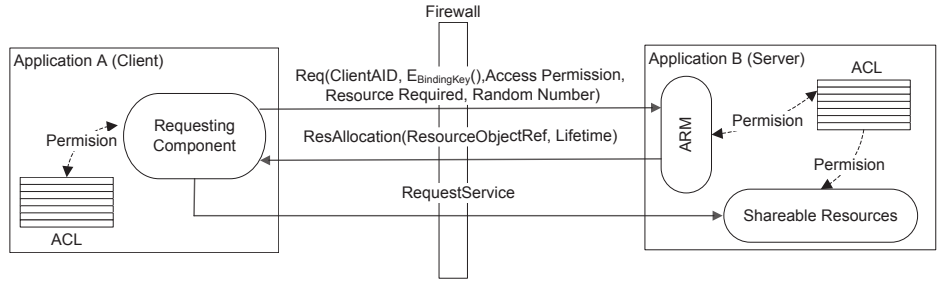
Fig. 7. Application Shareable Resource Access Request Process
