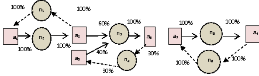
Fig. 5. The NDIG of the Database in Figure 2.
