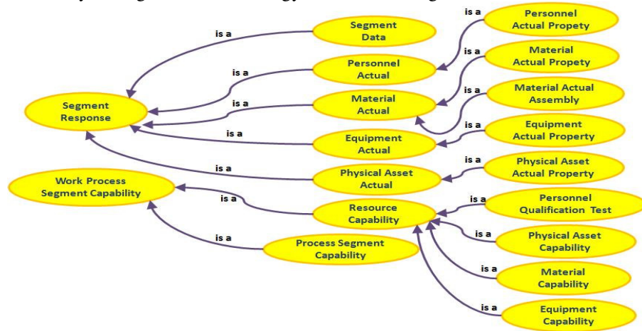
Fig. 3(b). The ISA S-95 Ontology – Resource Detail
