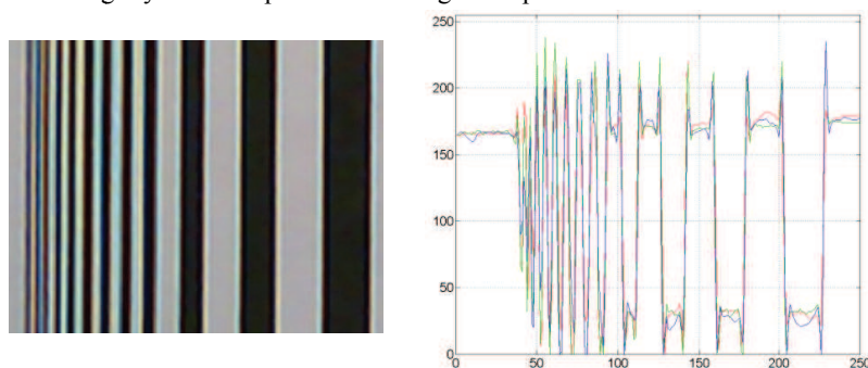
Fig. 6. Close-up on edge pattern showing colored artifacts.
