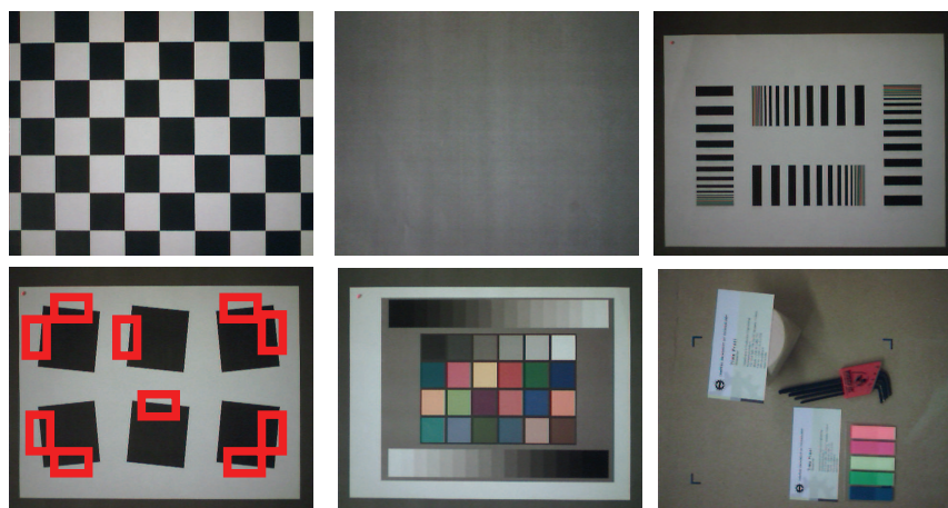
Fig. 2. Test targets imaged with OmniVision VGA camera module. Red rectangles on top of slanted square target indicate areas where edge sharpness was evaluated.
