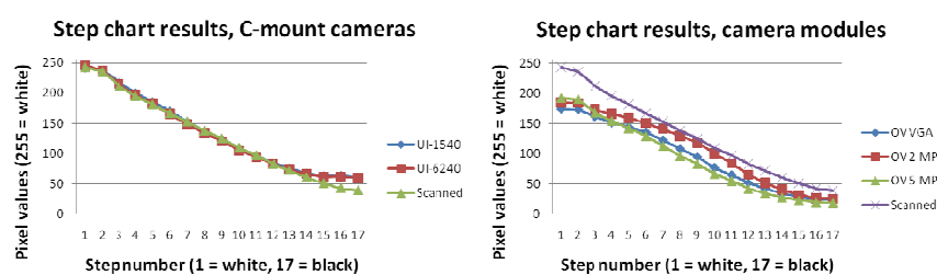
Fig. 7. Measured image brightnesses of 17 gray steps for C-mount cameras (on left) and for camera modules (on right).
