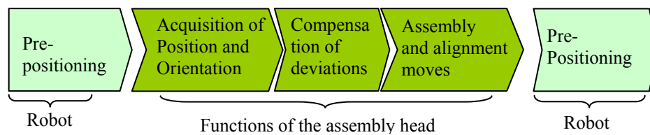
Fig. 1. Component handling process of a hybrid positioning device consisting of conventional robot and active assembly head
