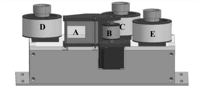
Fig. 5. The tape feeding system supplies adhesive gaskets automatically. Gaskets are provided on foil rolls and are covered by protection foils. Before hybrid bonding, one gasket is moved to the joining area while the protection foil is removed.
