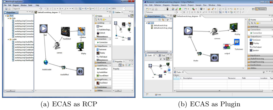
Fig. 1. Program appearance
