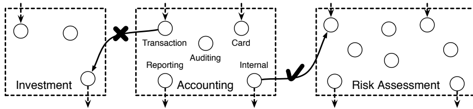
Fig. 2. Protection of flow categories within a bank. Flow categories define boundaries around data and specify which units can pass data over those boundaries. Transaction , as an input unit, cannot send data to the investment flow, while Internal , an output unit, can extract data from the flow.
