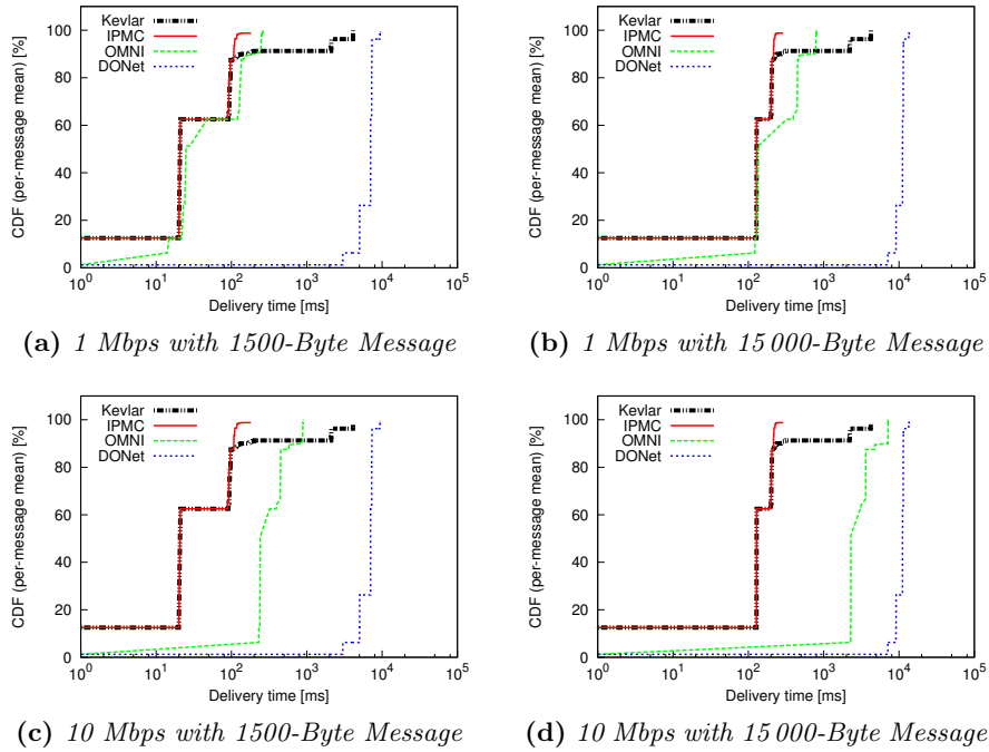
Fig. 8: Performance of simple applications (input traffic dependence). Performance comparison of multicast protocols for input traffic of various message size and data rate: each subfigure, corresponding to a different set of input parameter values, shows the CDF (per-message mean as in Fig. 7) of message delivery time. Space constraints preclude visualization of the remaining eleven experiments (specifically, data rates of 100 kbps, 300 kbps and 3 Mbps, and message size of 150 Bytes), with nearly identical results.
