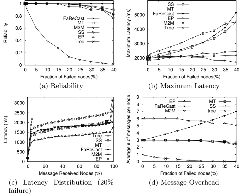
Fig. 3. Performance Comparison of FaReCasts( F_i=3, F_o=3 , M2M with Backup/L2L Dissemination) with other protocols under various failures with 100,000 nodes. (SS:SplitStream, MT:MultipleTree, EP:Epidemic)
