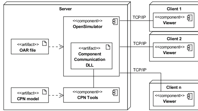
Fig. 6. Physical architecture of the APEX framework
