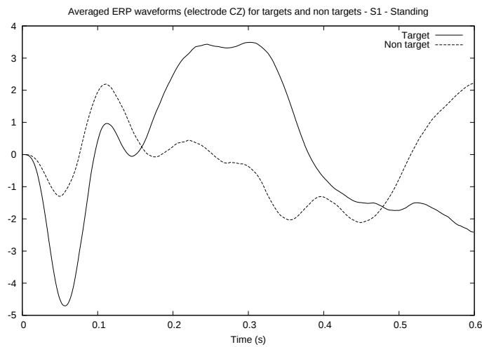
Fig. 7.8 An exemple of an average P300 ERP after a rare and relevant stimulus (Target). We can clearly observe the increase in amplitude about 300ms after the stimulus, as compared to the non-relevant stimulus (Non target).
