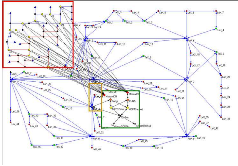
Fig. 4. Heterogeneous network supporting FISIR service.
