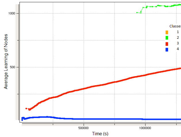
Fig. 5. Learning curve
