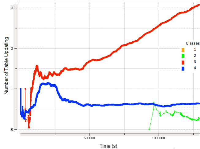
Fig. 6. Learning curve
