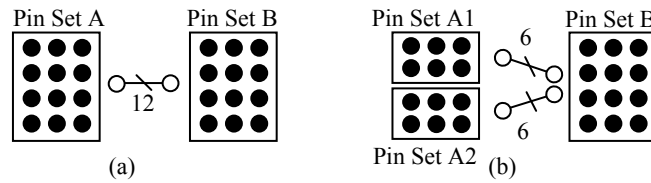
Fig. 6. Two pin assignment tasks for 12 two terminal nets. (a) 12 nets need an assignment to pins of sets A and B. (b) The nets of set B are to be assigned to two sets A1 and A2 and vice versa.
