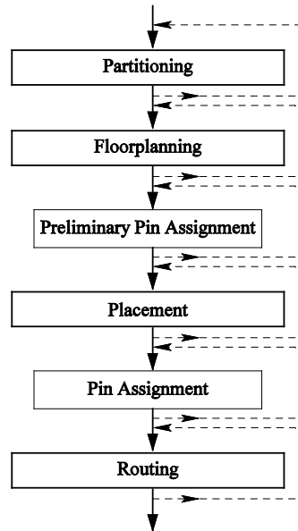
Fig. 3. Simplified physical design flow. The dashed arrows indicate iterations over the individual design steps.
