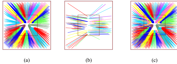
Fig. 11. Pin assignment for a single chip module using aggressive blending. (a) Fat pin assignment. (b) Assignment of remaining pins and nets. (c) The final pin assignment with 468 possible differential pairs is the combination of (a) and (b).
