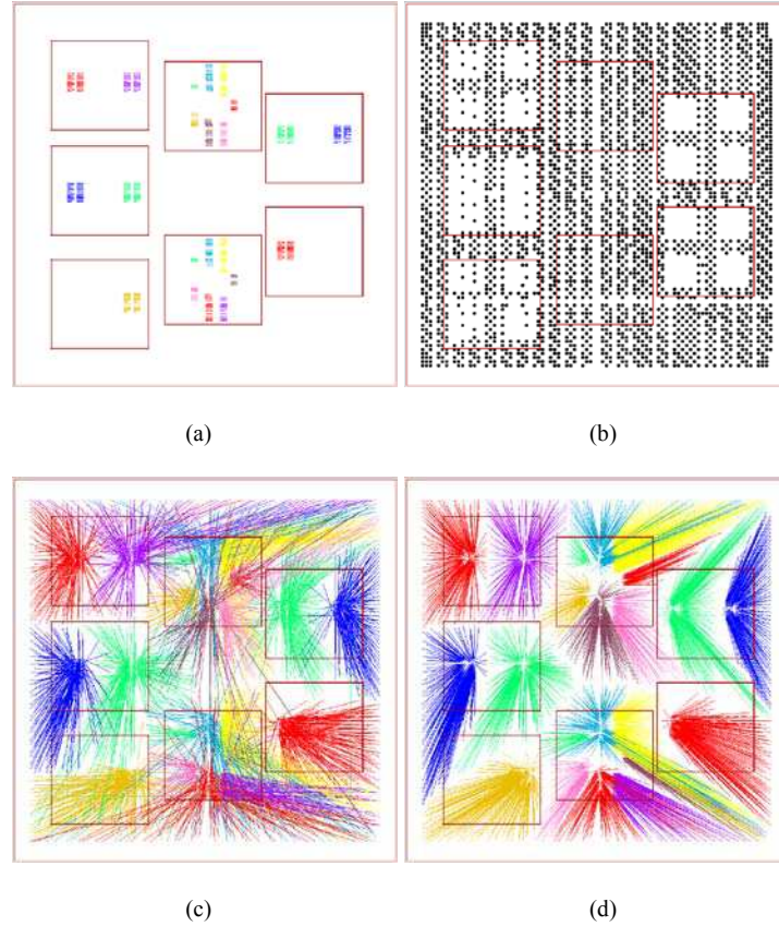
Fig. 1. Illustration of pin assignment with the I/O pins of seven chips (a) to be assigned to signals that connect a wiring substrate such as an MCM (b). The pin assignment based on the shortest Manhattan distances of the individual connections is depicted in (c) whereas (d) illustrates the pin assignment with minimum overall length of all Euclidean distances ( flylines ).
