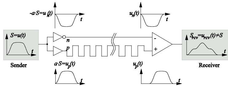
Fig. 5. Effect of unmatched propagation delays of a differential pair.
