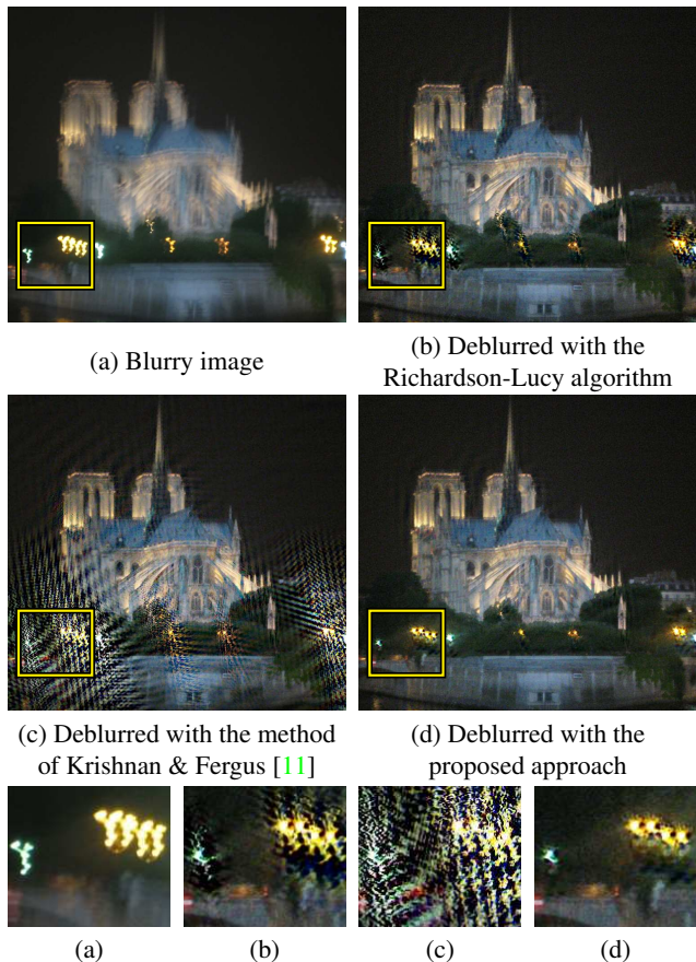
Figure 1. Deblurring in the presence of saturation. Existing deblurring methods, such as those in (b) & (c), do not take account of saturated pixels. This leads to large and unsightly artifacts in the results, such as the “ringing” around the bright lights in the zoomed section. Using the proposed method (d), the ringing is greatly reduced and the quality of the deblurring improved.
