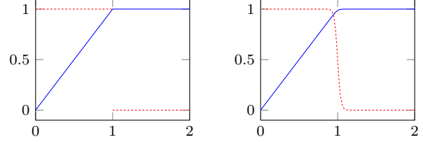
(a) Ideal saturation function (b) Smooth, differentiable saturation function
