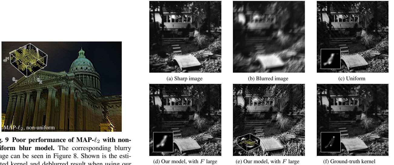
Fig. 10 Blind deblurring of a real uniform blur. A real camera shake blur (a–b) from the dataset of Levin et al. (2009), deblurred using kernels estimated with the marginalization algorithm. We show deblurred results and kernels for four cases; (c) uniform blur using original algorithm of Fergus et al., (d) our model with a large focal length F and no in-plane rotation ( \theta_Z = 0 ), (e) our approach with a large focal length F but with \theta_Z unconstrained, and (f) the ground-truth (uniform) kernel, provided with the dataset. Note that (d) is indistinguishable from (c), apart from a translation, and that the kernel in (d), while not perfect, does have the same diagonal shape as the true blur, with the non-zeros centered around a single value of \theta_Z
