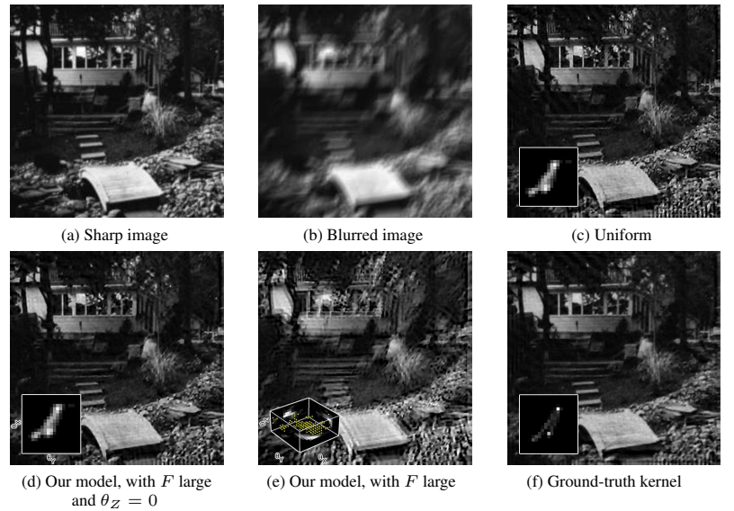
Fig. 10 Blind deblurring of a real uniform blur. A real camera shake blur (a–b) from the dataset of Levin et al. (2009), deblurred using kernels estimated with the marginalization algorithm. We show deblurred results and kernels for four cases; (c) uniform blur using original algorithm of Fergus et al., (d) our model with a large focal length F and no in-plane rotation ( \theta_Z = 0 ), (e) our approach with a large focal length F but with \theta_Z unconstrained, and (f) the ground-truth (uniform) kernel, provided with the dataset. Note that (d) is indistinguishable from (c), apart from a translation, and that the kernel in (d), while not perfect, does have the same diagonal shape as the true blur, with the non-zeros centered around a single value of \theta_Z
