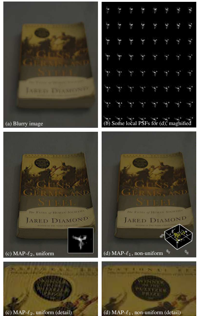
Fig. 6 Blind deblurring of real camera shake, example 2. The result of blind deblurring on a real camera shake image (a), captured with a shutter speed of 1 second, using the MAP approach of Cho and Lee with both the uniform and non-uniform blur models. Also shown in (b) are some of the local PSFs generated from the blur kernel in (d) at various points in the image. In the blurry image, most of the text on the book cover is too blurred to read. Deblurring the image with the uniform blur model (c) allows some of the text on the cover of the book to be read, however, after deblurring with our non-uniform model (d), all but the smallest text becomes legible. The blur kernel in (d) covers \pm 0.4^\circ in \theta_X and \theta_Y , and \pm 0.9^\circ in \theta_Z
