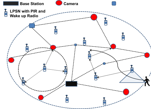
Fig. 2: Ultra-low power sensor network overlayed on an existing WSN.
