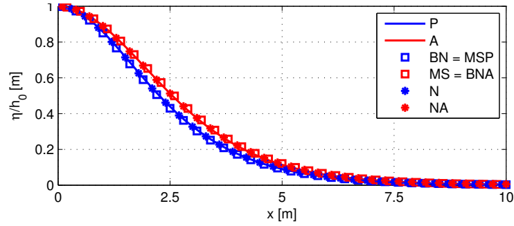
Figure 5: Semi-analytical exact solitary waves for the Boussines models of the paper.
