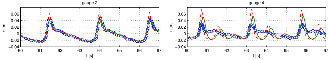
Figure 23: Propagation over a submerged bar, case (b); data in gauge 2 (left) and gauge 4 (right): experimental data [3] ( \circ ), BNA model ( — ), BN model ( - - ).
