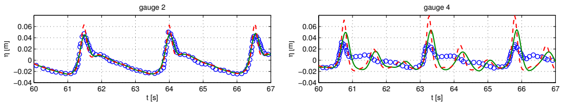
Figure 22: Propagation over a submerged bar, case (b); data in gauge 2 (left) and gauge 4 (right): experimental data [3] ( \circ ), A model (—), P model (- -).
