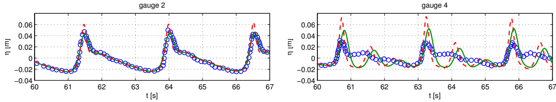
Figure 24: Propagation over a submerged bar, case (b); data in gauge 2 (left) and gauge 4 (right): experimental data [3] ( \circ ), MS model ( — ), MSP model ( - - ).
