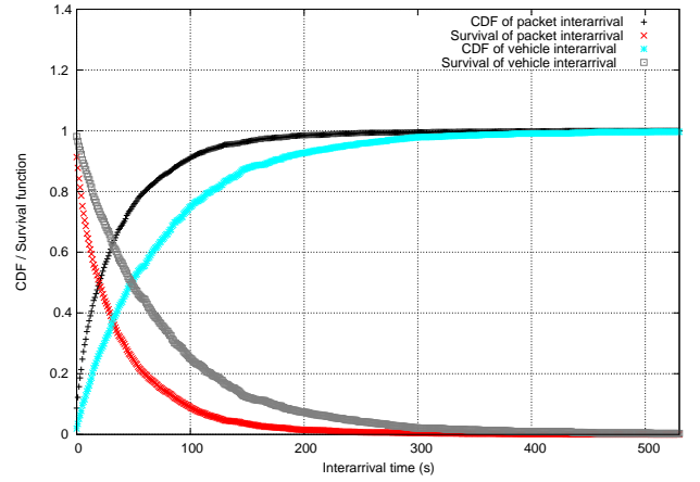
Figure 4: The CDF and survival function of vehicle and packet interarrival times of 24 in-ground parking sensors
