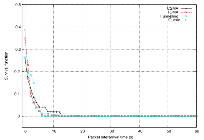
Figure 10: The survival function of packet interarrival time on the gateway side: Mesh
