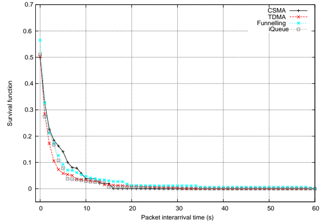
Figure 8: The survival function of packet interarrival time on the gateway side: Crossroad
