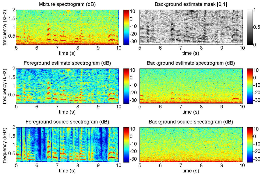
Fig. 6 Noise/speech separation using REPET-SIM. The mixture is a female speaker (foreground) speaking in a town square (background). The square has repeating noisy elements (passers-by and cars) that happen intermittently. The spectrograms and the mask are shown for 5 seconds and up to 2 kHz. The file is dev_Sql_Co_B from the task of two-channel mixtures of speech and real-world background noise of the Signal Separation Evaluation Campaign (SiSEC) 8 .
