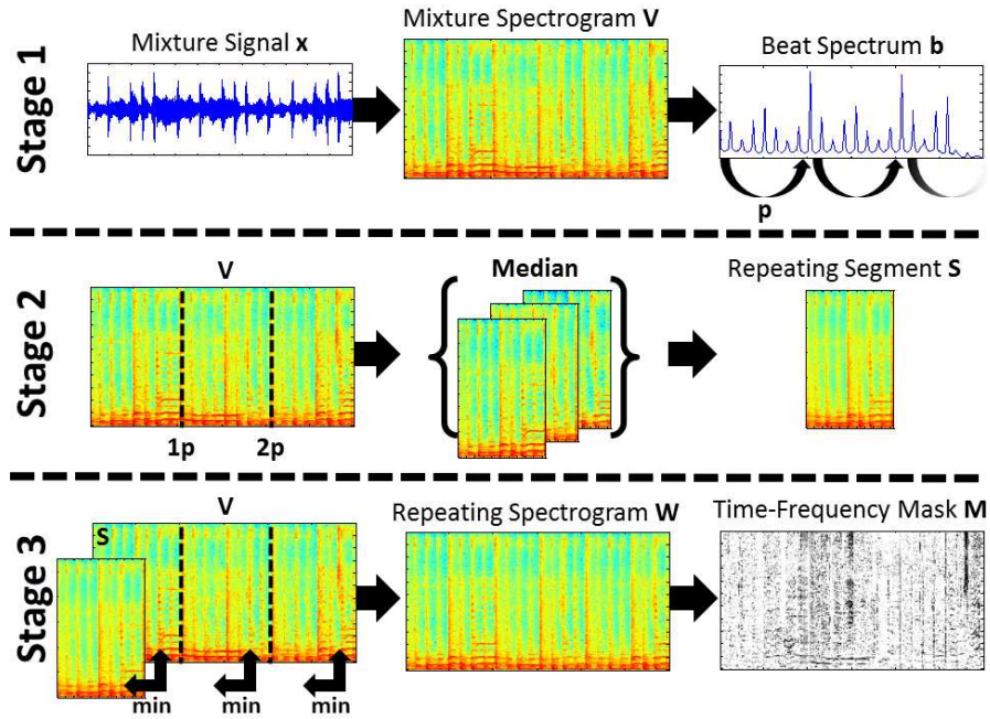
Fig. 1 Overview of the original REPET. Stage 1: calculation of the beat spectrum b and estimation of a repeating period p . Stage 2: segmentation of the mixture spectrogram V and calculation of the repeating segment model S . Stage 3: calculation of the repeating spectrogram model W and derivation of the soft time-frequency mask M .
