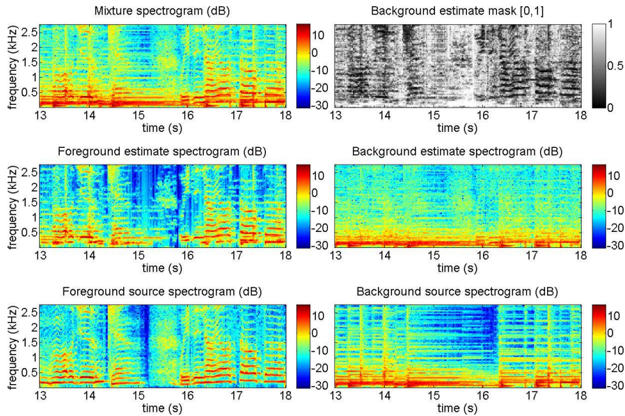
Fig. 4 Music/voice separation using the adaptive REPET. The mixture is a male singer (foreground) singing over a guitar and drums accompaniment (background). The guitar has a repeating chord progression that changes around 15 seconds. The spectrograms and the mask are shown for 5 seconds and up to 2.5 kHz. The file is Another Dreamer - The Ones We Love from the task of professionally produced music recordings of the Signal Separation Evaluation Campaign (SiSEC) 6 .
