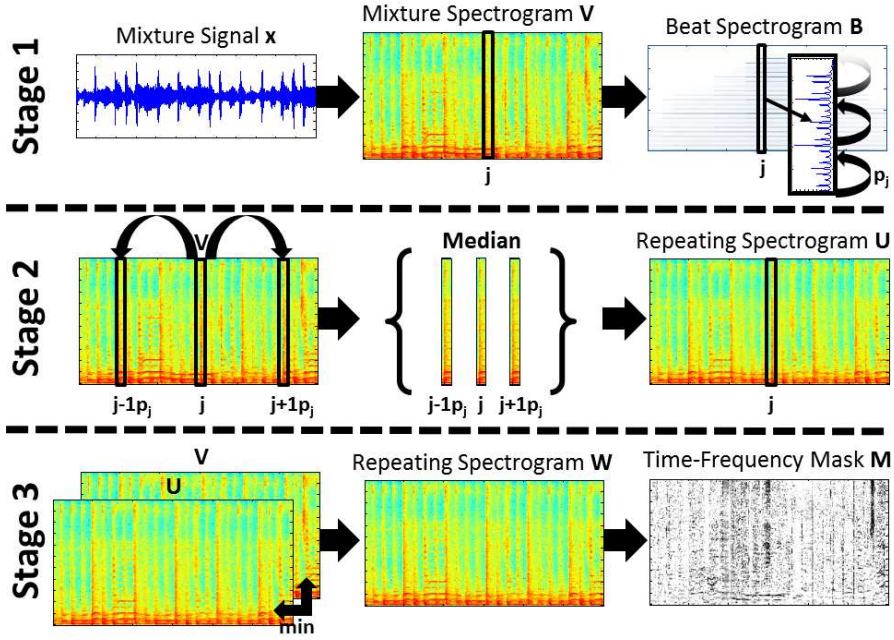
Fig. 3 Overview of the adaptive REPET. Stage 1: calculation of the beat spectrogram B and estimation of the repeating periods p_j 's. Stage 2: filtering of the mixture spectrogram V and calculation of an initial repeating spectrogram model U . Stage 3: calculation of the refined repeating spectrogram model W and derivation of the soft time-frequency mask M .
