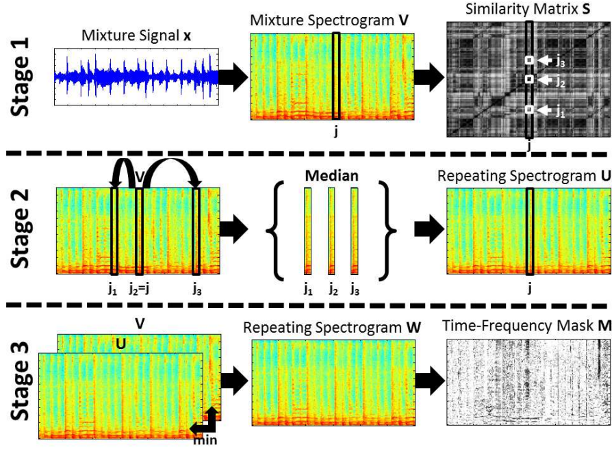
Fig. 5 Overview of REPET-SIM. Stage 1 : calculation of the similarity matrix S and estimation of the repeating elements j_k 's. Stage 2 : filtering of the mixture spectrogram V and calculation of an initial repeating spectrogram model U . Stage 3 : calculation of the refined repeating spectrogram model W and derivation of the soft time-frequency mask M .
