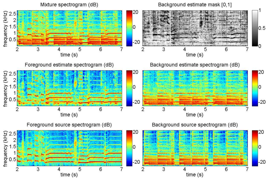
Fig. 2 Music/voice separation using the original REPET. The mixture is a female singer (foreground) singing over a guitar accompaniment (background). The guitar has a repeating chord progression that is stable along the song. The spectrograms and the mask are shown for 5 seconds and up to 2.5 kHz. The file is Tamy - Que Pena Tanto Faz from the task of professionally produced music recordings of the Signal Separation Evaluation Campaign (SiSEC) 3 .
