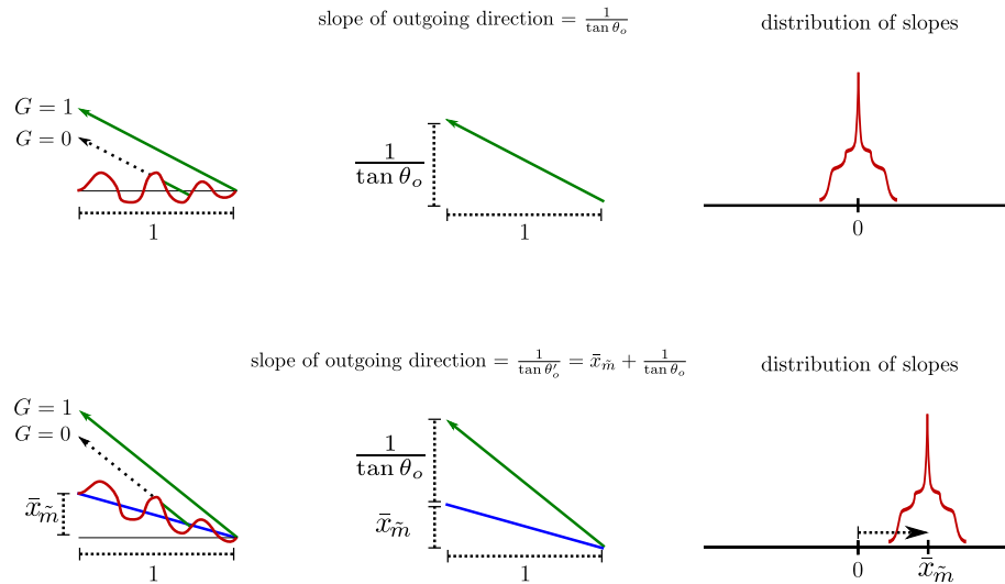
Figure 15. Vertical shearing of a 1D configuration. This does not change masking probability G_1 , but all of the slopes of the configuration are offset by a constant factor \bar{x}_{\bar{m}} . This includes the slopes of the microsurface as well as the slope associated with the outgoing direction. The distribution of slopes is shifted by an offset \bar{x}_{\bar{m}} and is no longer centered around 0.
