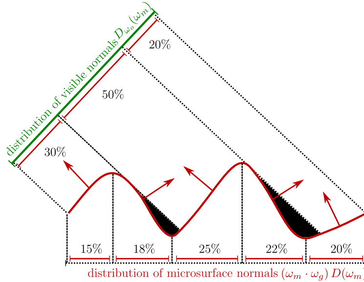
Figure 5. The distribution of microsurface normals (\omega_m \cdot \omega_g)D(\omega_m) is an intrinsic surface property, while the distribution of visible normals D_{\omega_o}(\omega_m) is view dependent.
