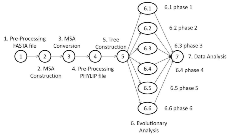
Figure 2: SciEvol workflow [82].
