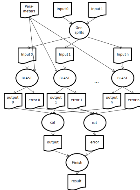
Figure 5: BLAST workflow [3].
