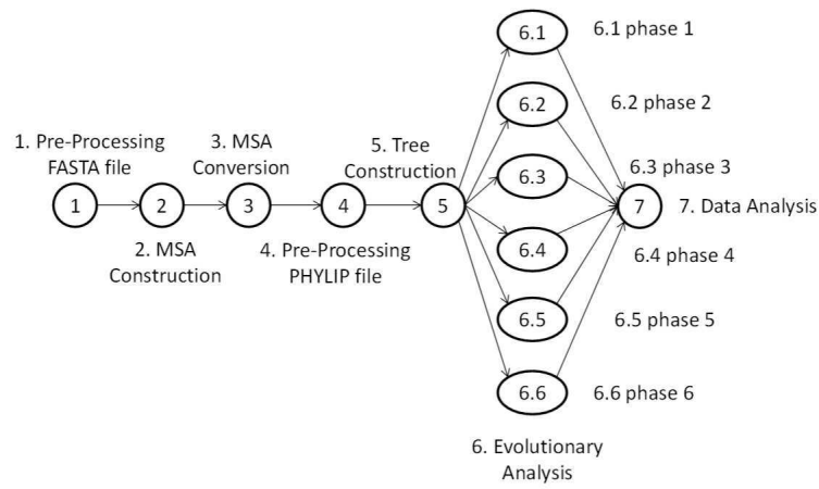
Figure 2: SciEvol workflow [82].
