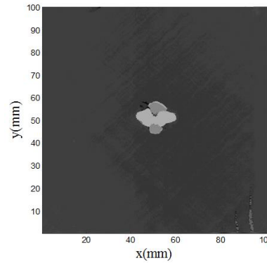
Figure 7. Damage evaluation using immersion ultrasonic C-scan method
