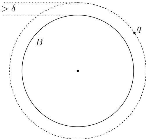
Figure 4: A Delaunay simplex \sigma is \delta -protected if it has a Delaunay ball B_{\mathbb{R}^m}(c; r) such that \overline{B_{\mathbb{R}^m}(c; r + \delta)} \cap (\mathcal{P} \setminus \sigma) = \emptyset .
