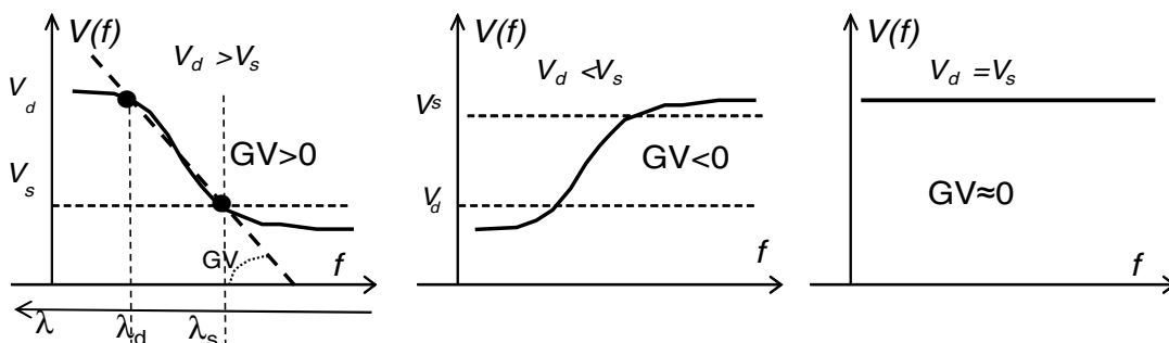
Figure 2. Three basic shapes of dispersion characteristics V(f) and corresponding GV values
