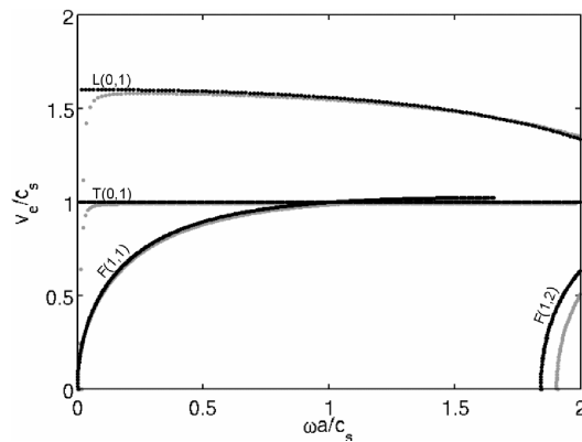
Figure 1 : Normalized energy velocity dispersion curves of isolated wires (i.e. uncoupled from each other). Black: central cylindrical wire, gray: peripheral helical wire.
