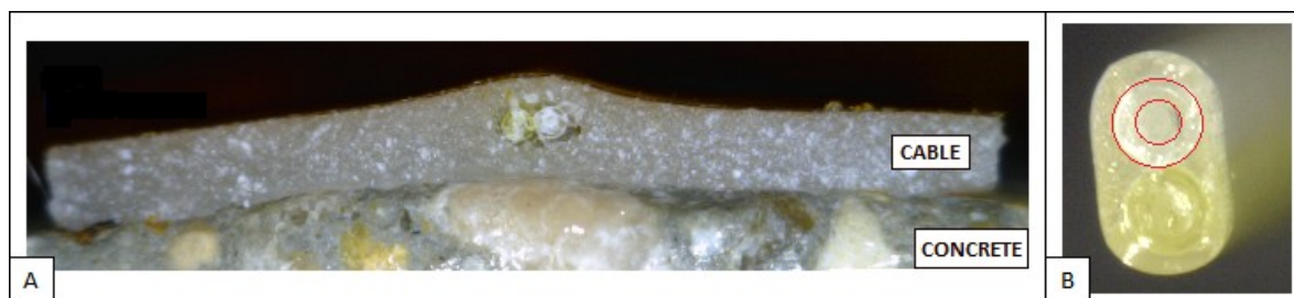
Figure 1: A – View of the cross-section of the cable stuck to the concrete surface. B – Zoom of the cable core, where two fibers and their primary coatings are assembled into a polymer matrix
