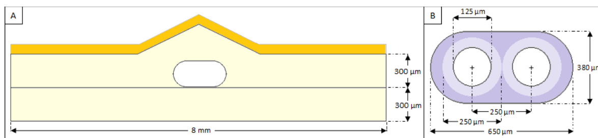
Figure 4: Simplified geometry of the model: A – Total section of the cable. B – Zoom of the core structure.
